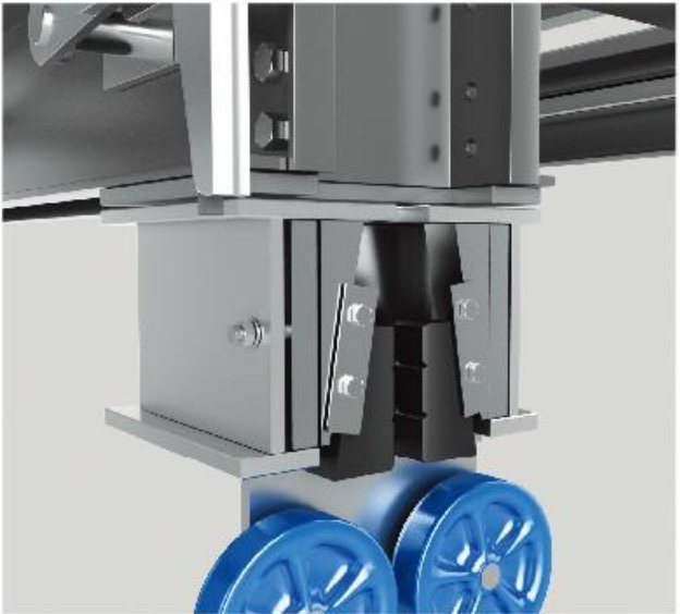
SAFETY GEAR
